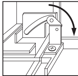
Self Locking Double Cam Action Hinges
