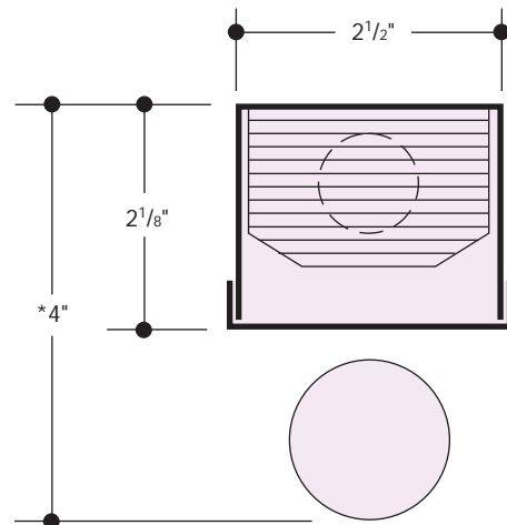
Dimensions shown are with T-12 lamp. * Minus 1/4" for OCTRON T-8 lamp.
