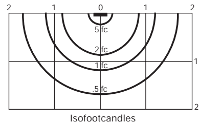
Multiples of mounting height 75W incandescent @ 8' mounting height
